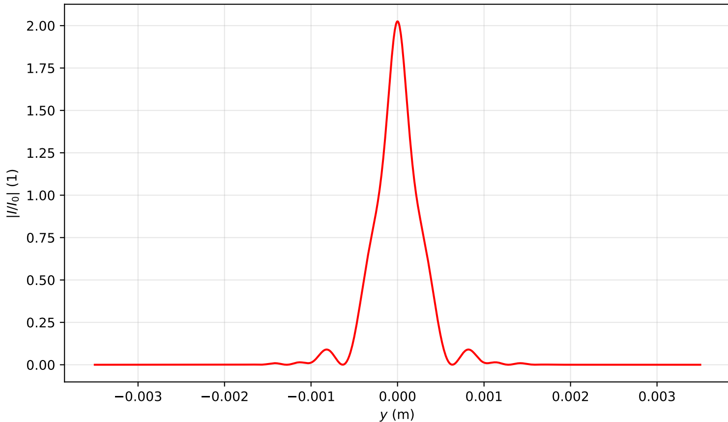
Intensity profile I(x=0, y, z=1.194)/I_0 , P_{in}=3.5P_{cr} , artificial time
